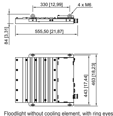
Floodlight without cooling element, with ring eyes
