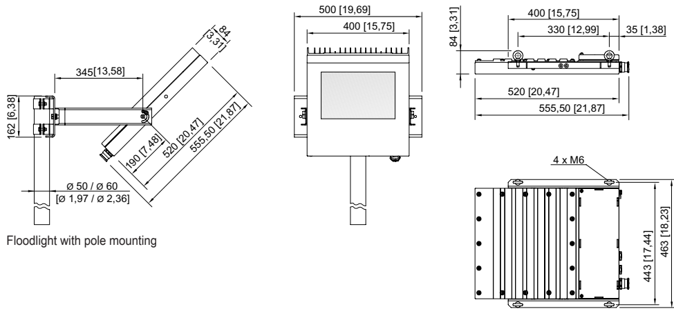
Mounting bracket
