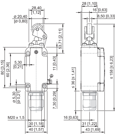
Roller lever 8074/2-5-WH-40
