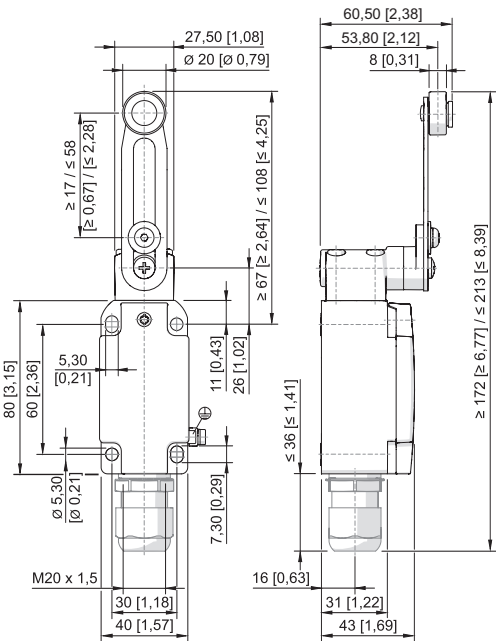
Schwenkhebel 8074/2-4-DS-40
