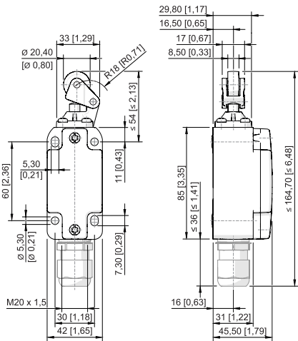
Rollenhebel 8070/2-5-WH-U60
