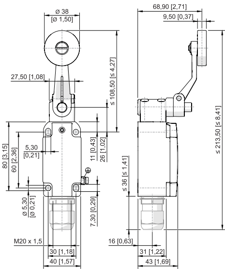
Stangenhebel 8074/2-2-DL-40
