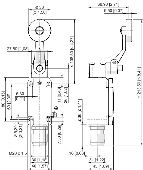
Stangenhebel 8074/2-5-DL-40
