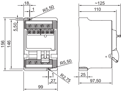
Fi-Schutzschalter, 4-polig, 8562/54-...
