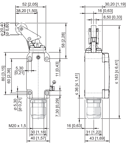
Rollenhebel 8074/2-.-WPH-40
